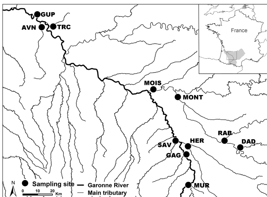
Fig. 1. Selected sampling sites throughout the Garonne river basin (grey area in insert map). Sampling site abbreviations as explained in Table 2. Main tributaries flow towards/into the Garonne River, which flows from South to Northwest.
