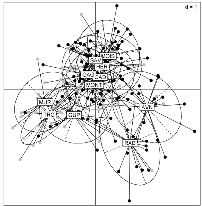
Fig. 3. Two dimensional distribution of the gudgeon individuals from the 11 sampling sites after Linear Discriminant Analysis (LDA) based on the right-side morphometric measurements (I to XVII, see Fig. 2); ellipses group individuals from each sampling site (Monte-Carlo test after 1000 permutations: p = 0.001 ). Point shading indicates the inferred genetic cluster to which individuals belong when q (fractional membership) > 70\% (identified using STRUCTURE; K = 2 ; for details see Section 2.4). Sampling site abbreviations as explained in Table 2.
