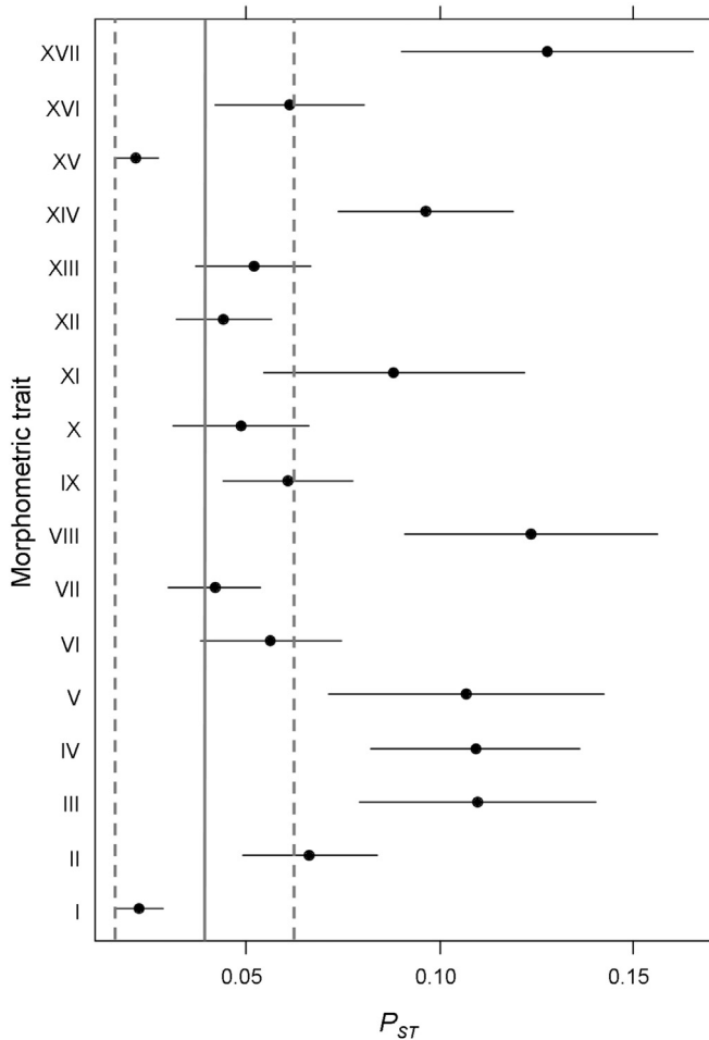
Fig. 4. Indices quantifying the genetic divergence of natural populations ( P_{ST} ) for the morphometric traits I to XVII (see Fig. 2) with the data of all 11 populations, and indices quantifying the among-population divergence between genes ( F_{ST} ) coding for quantitative traits. P_{ST} = mean (black point) and 95% confidence interval (horizontal lines); F_{ST} = mean of all population and loci (solid vertical line) and 95% confidence interval (dashed vertical lines).
