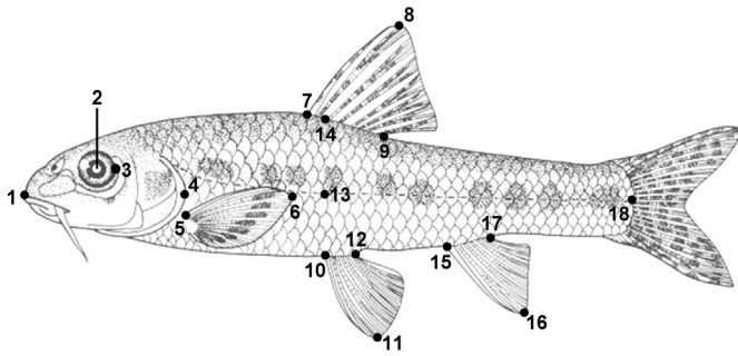
Fig. 2. Placement of landmarks on a gudgeon specimen sketch (Illustration by Susan Laurie Bourque, reproduced with permission from the Canadian Museum of Nature, Ottawa, Canada). Footnote: The following morphometric traits were measured: I (1–2), II (2–3), III (1–4), IV (4–5), V (5–6), VI (1–10), VII (10–11), VIII (10–12), IX (13–14), X (1–18), XI (1–7), XII (7–8), XIII (7–9), XIV (15–16), XV (15–17), XVI (1–15), XVII (10–14).
