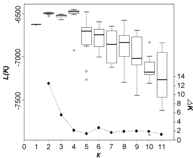
Fig. 5. Identification of population genetic structure based on Bayesian clustering. Given are posterior probabilities L(K) (box plots) and second order rate of change in the likelihood of K ( \Delta K , full dots) according to the number of genetic clusters ( K ). See Section 2.4. for analysis details.
